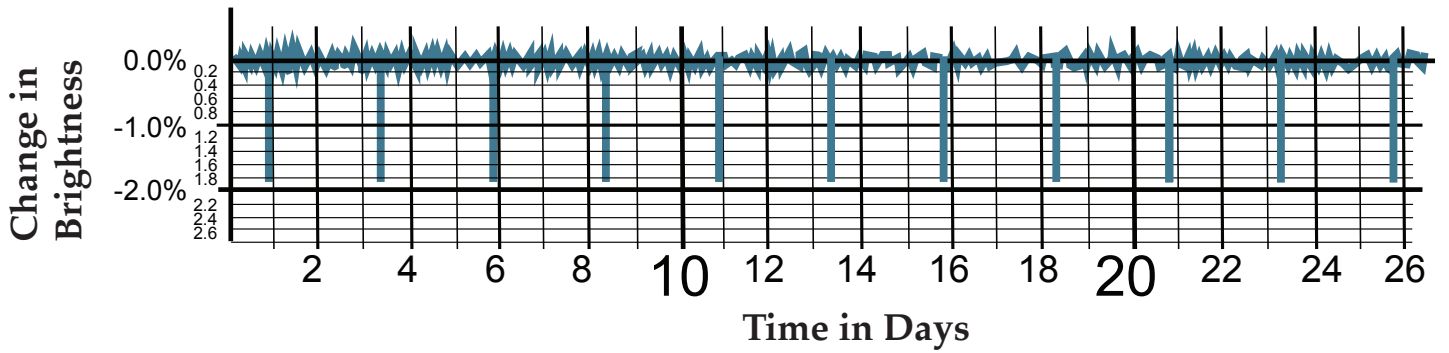
Kepler-1b (TrES-2)
