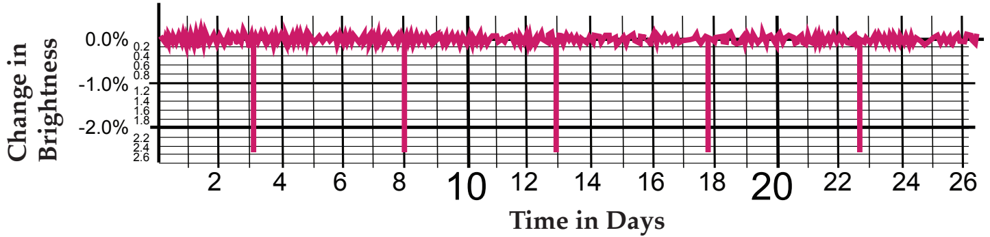
Kepler-7b
