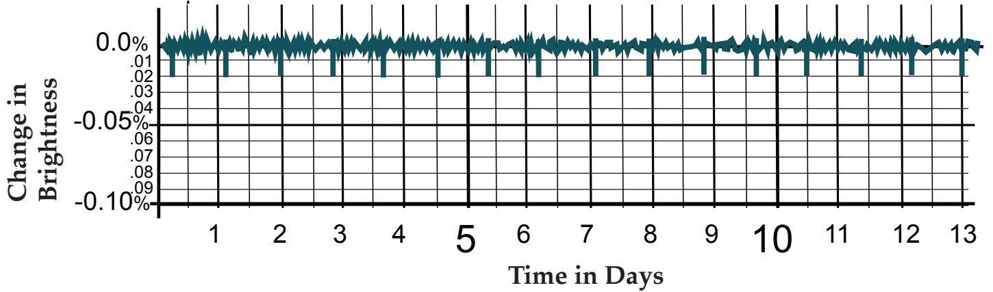
Kepler-10b
