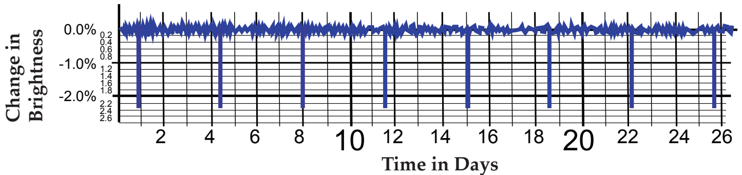
Kepler-8b
