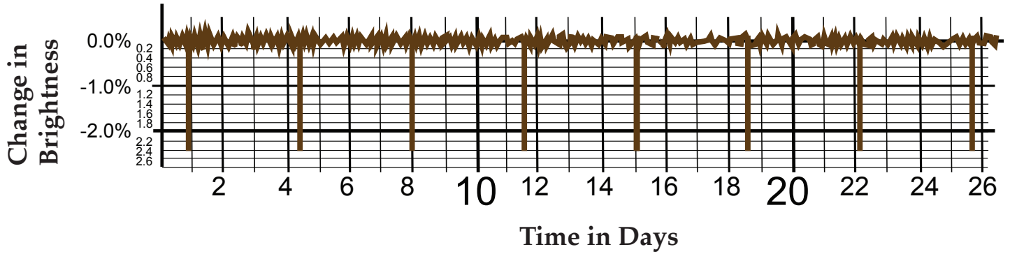
Kepler-6b
