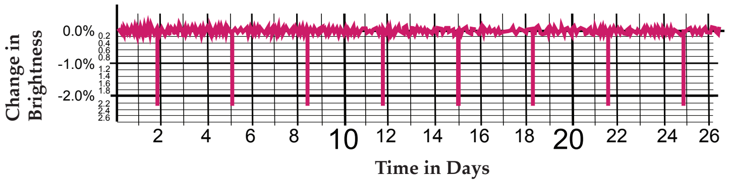
Kepler-6b
