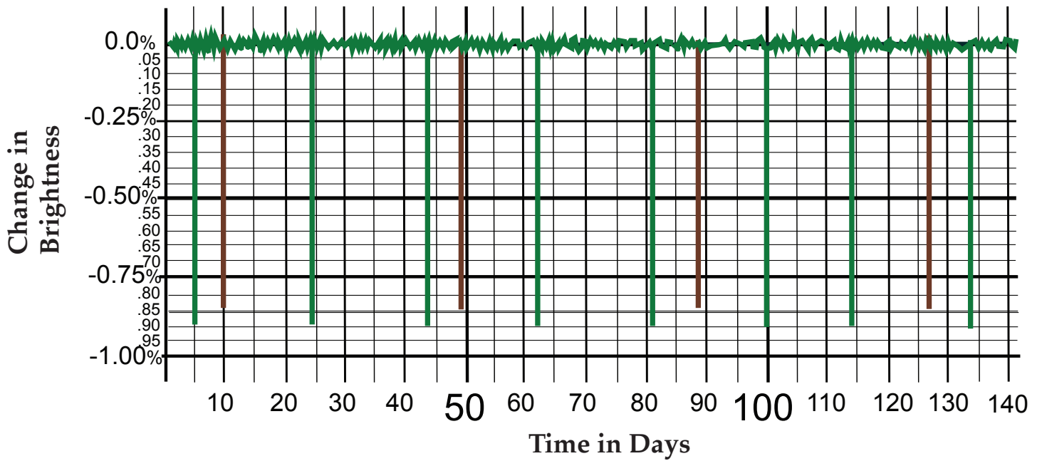
Kepler-9b, 9c
